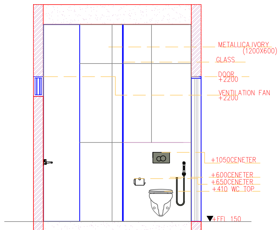
SECTIONAL ELEVATION - WALL A
