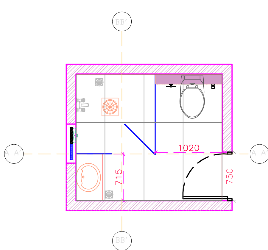
TOILET: FURNITURE LAYOUT
