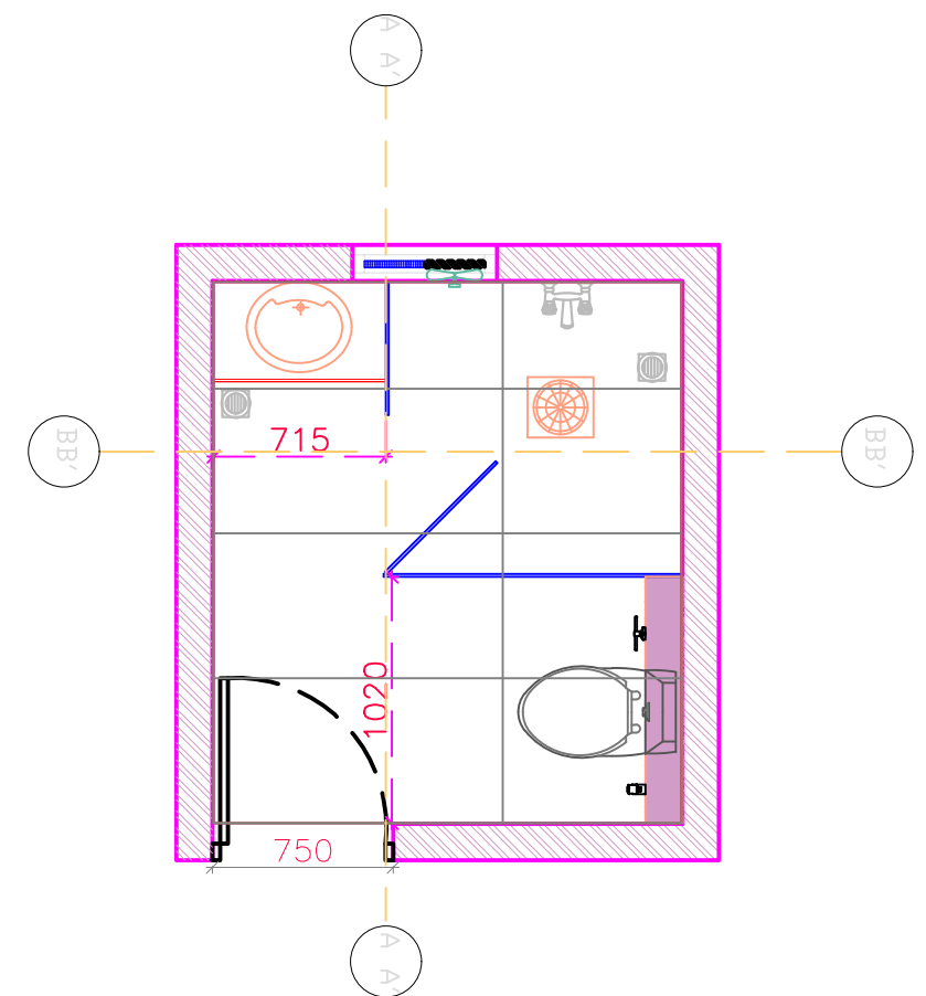
SECTIONAL PLAN - WALL B
