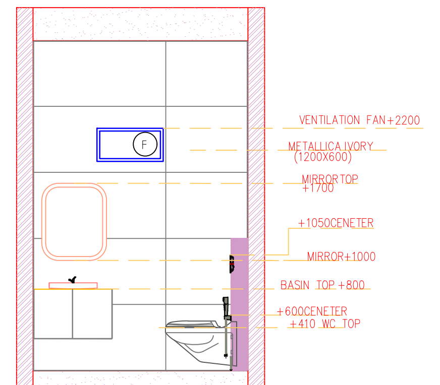
SECTIONAL ELEVATION - WALL B
