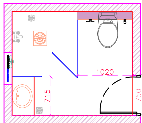
TOILET: FIXTURES LAYOUT
