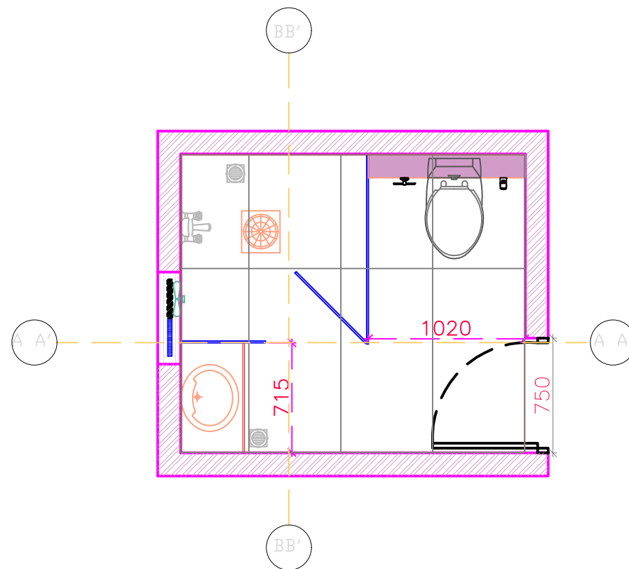
SECTIONAL PLAN - WALL A
